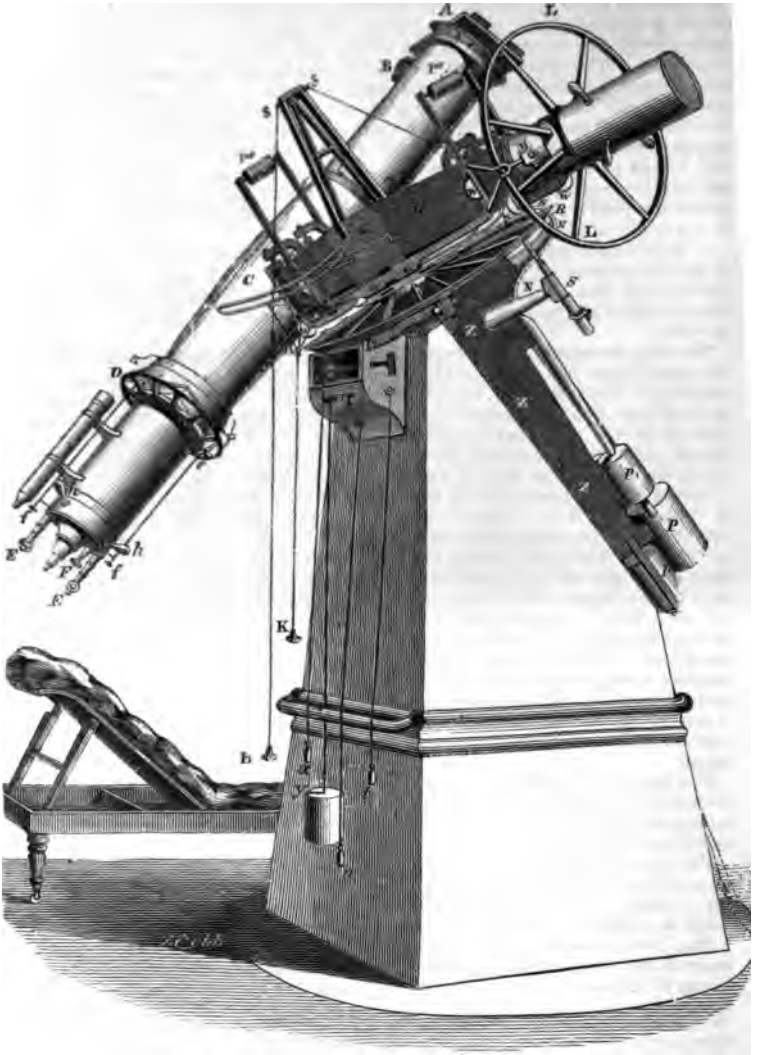
THE HELIOMETER OF THE RADCLIFFE OBSERVATORY.
